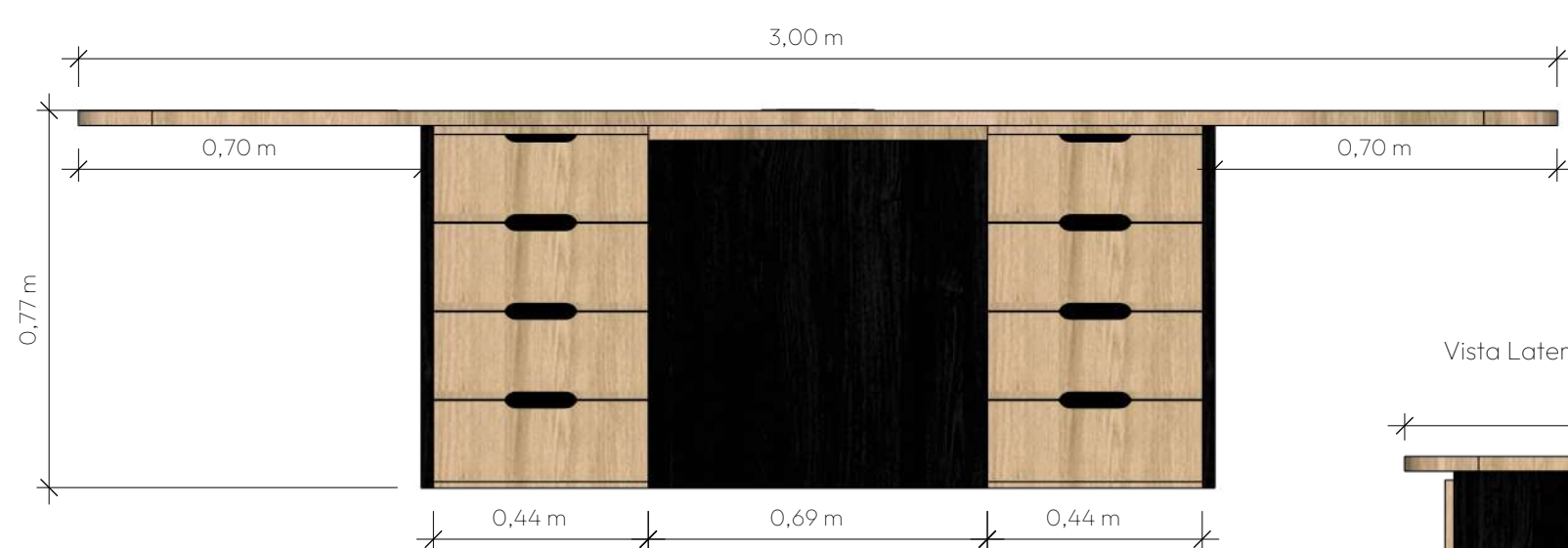
Vista Frontal
