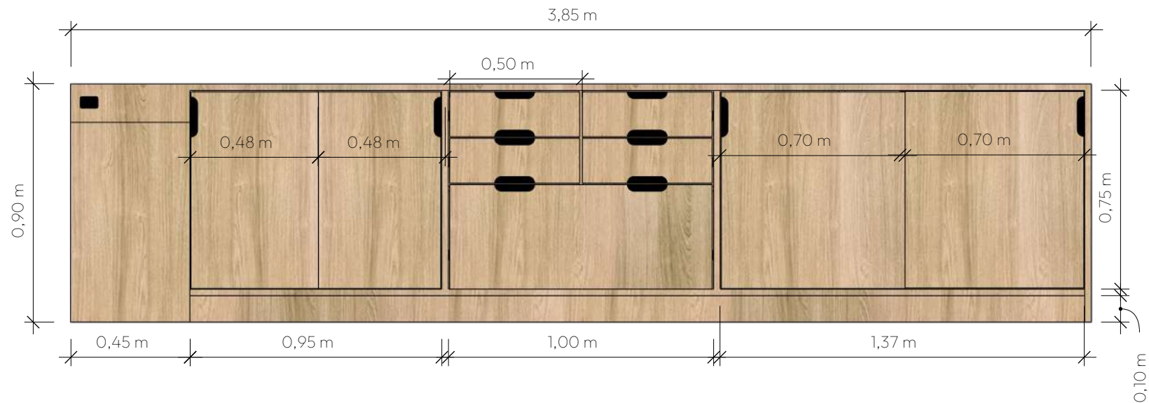
Vista Frontal
